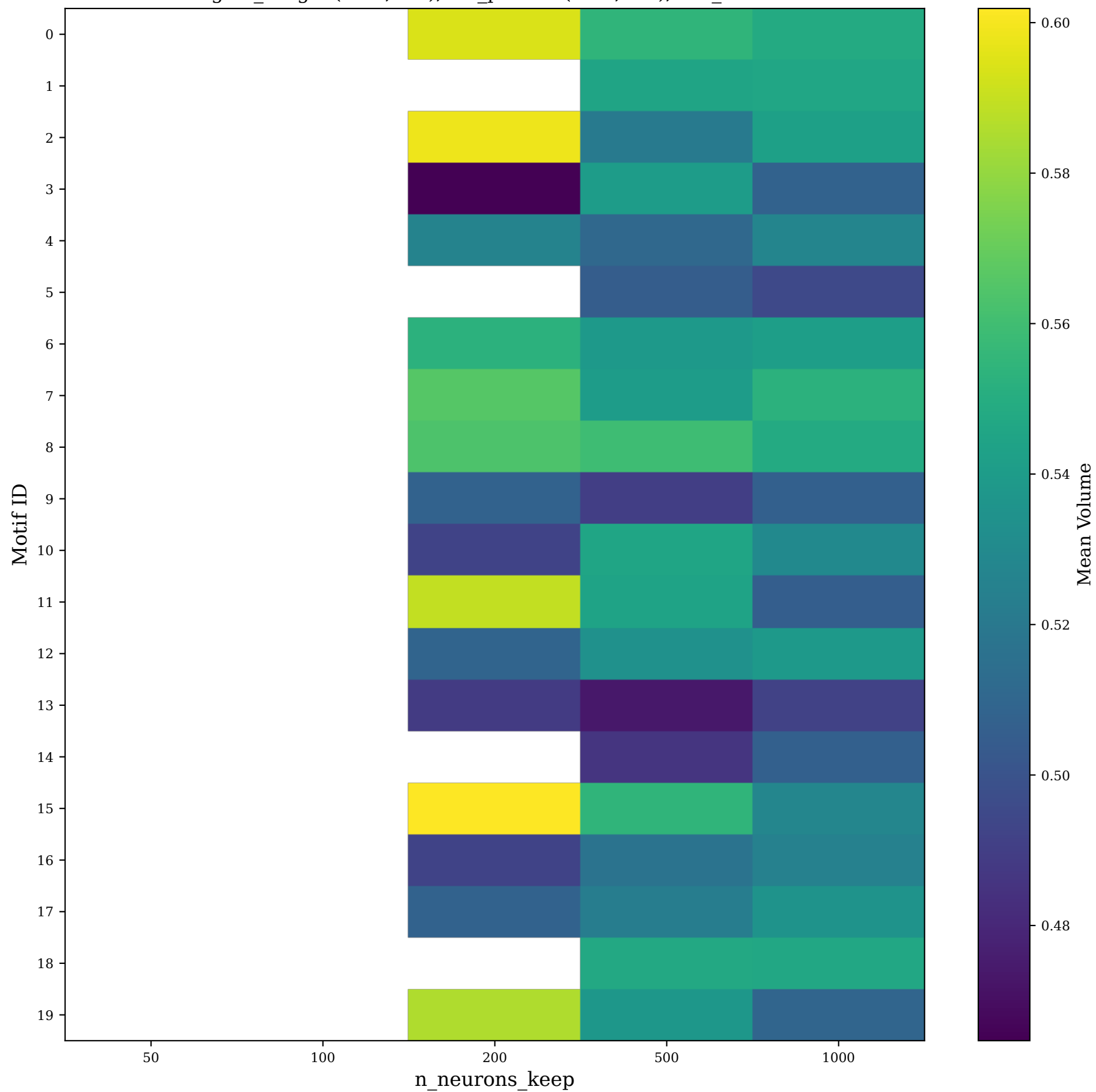
Mean Volumes of High-Correlation Motifs (corr > 0.4) sigma_range: (0.02, 0.4), vol_param: (0.07, 0.9), rho_vol: 0.7
